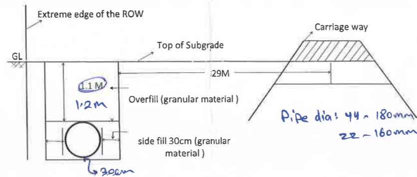
Pipeline Along the Road section @Y-Y and Z-Z
