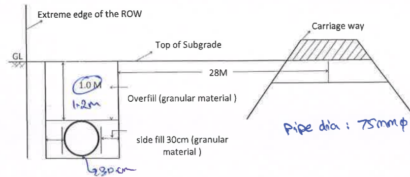
Pipeline Along the Road section @X-X
