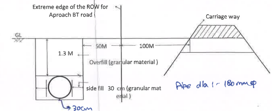
Pipeline Along NH and across BT Road section @W-W
